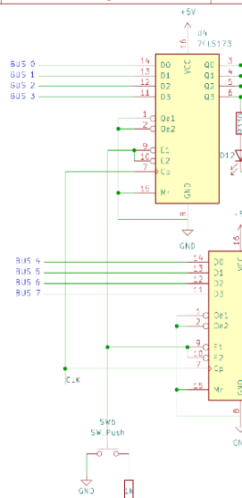
B-Register
